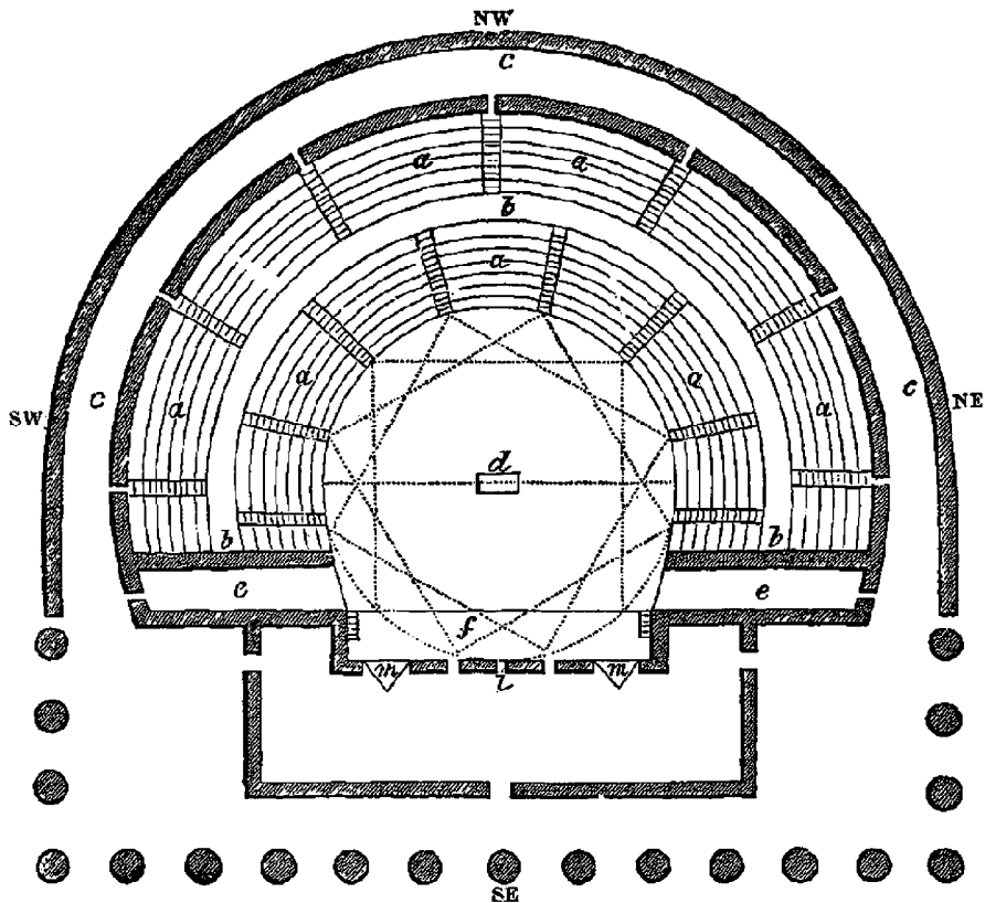
SE Plan of a Greek Theatre.
