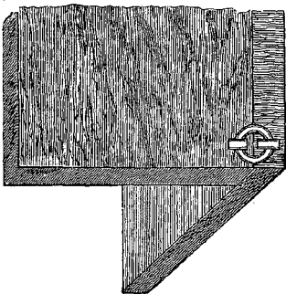
Top and Bottom Parts of Corner Boards (according to Paine).
