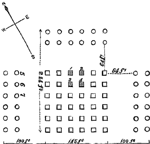
Plan of the Great Palace at Susa.
