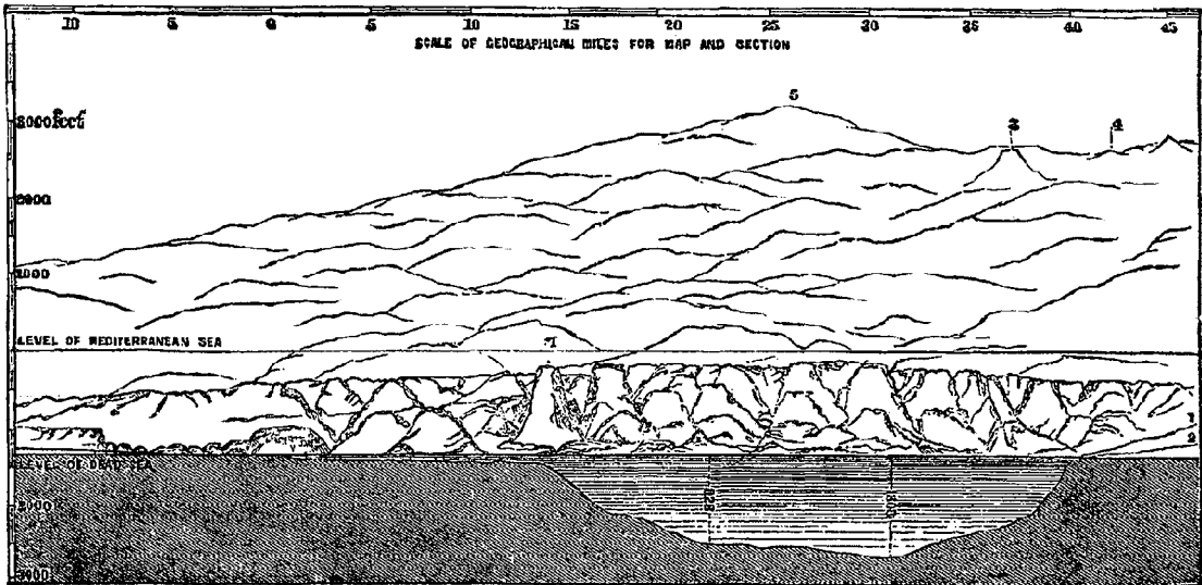
Section of the Dead Sea from North to South.
