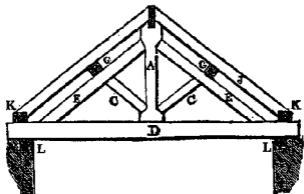
King-post Roof.
