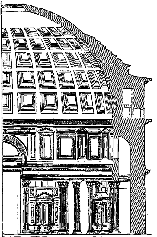
Half Section of Pantheon (from Fergusson).
