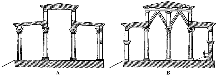
Fig. 2. Conjectural Sections of "the House of the Cedars of Lebanon," according to Ferguson.
