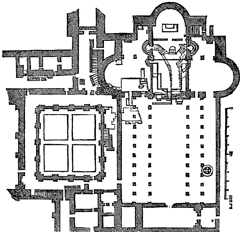
Plan of the Church of the Nativity at Bethlehem. (The dotted lines indicate the grottoes in the crypt below the church.)
