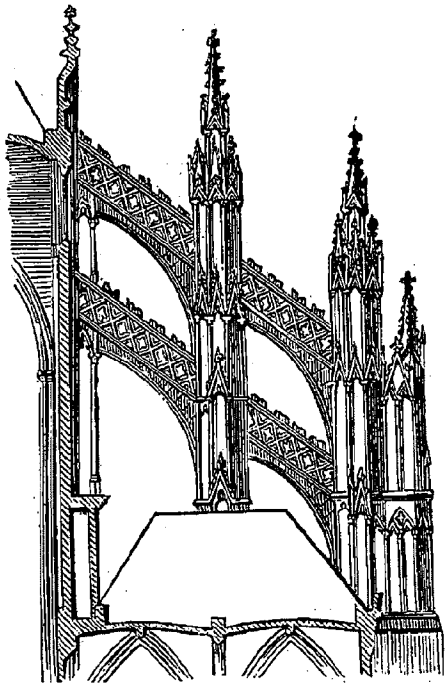
Fig. 5. Flying-buttress of the Cathedral at Cologne
