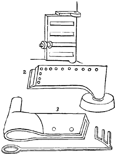
Ancient Egyptian Bolt, Hinges, and Key to a Door
