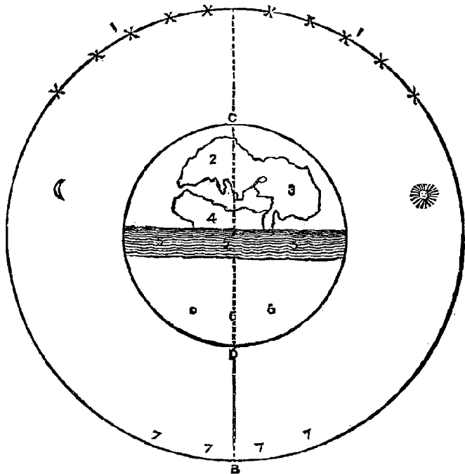
Diagram of Ancient Cosmology.
