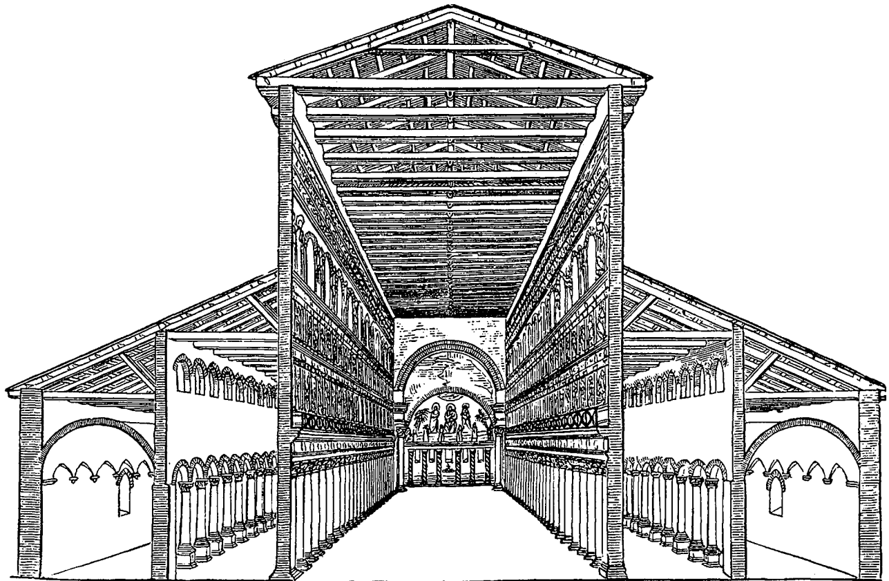
Section of the Basilica of St. Peter at Rome, erected in the Time of Constantine.
